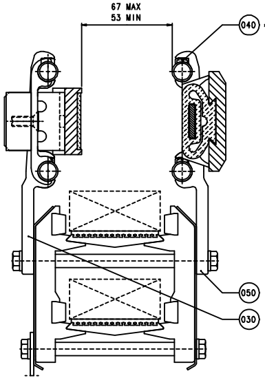
D - D, B68/R68
