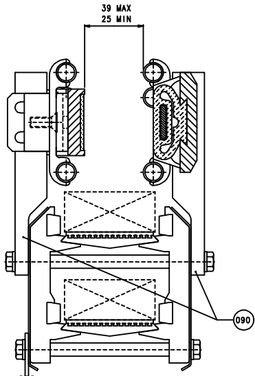
D - D, B40
