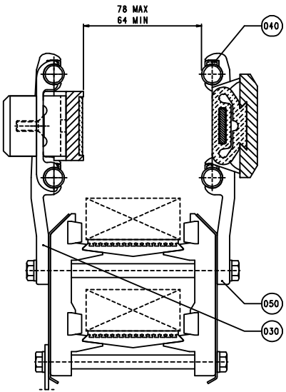
D - D, B79/R79
