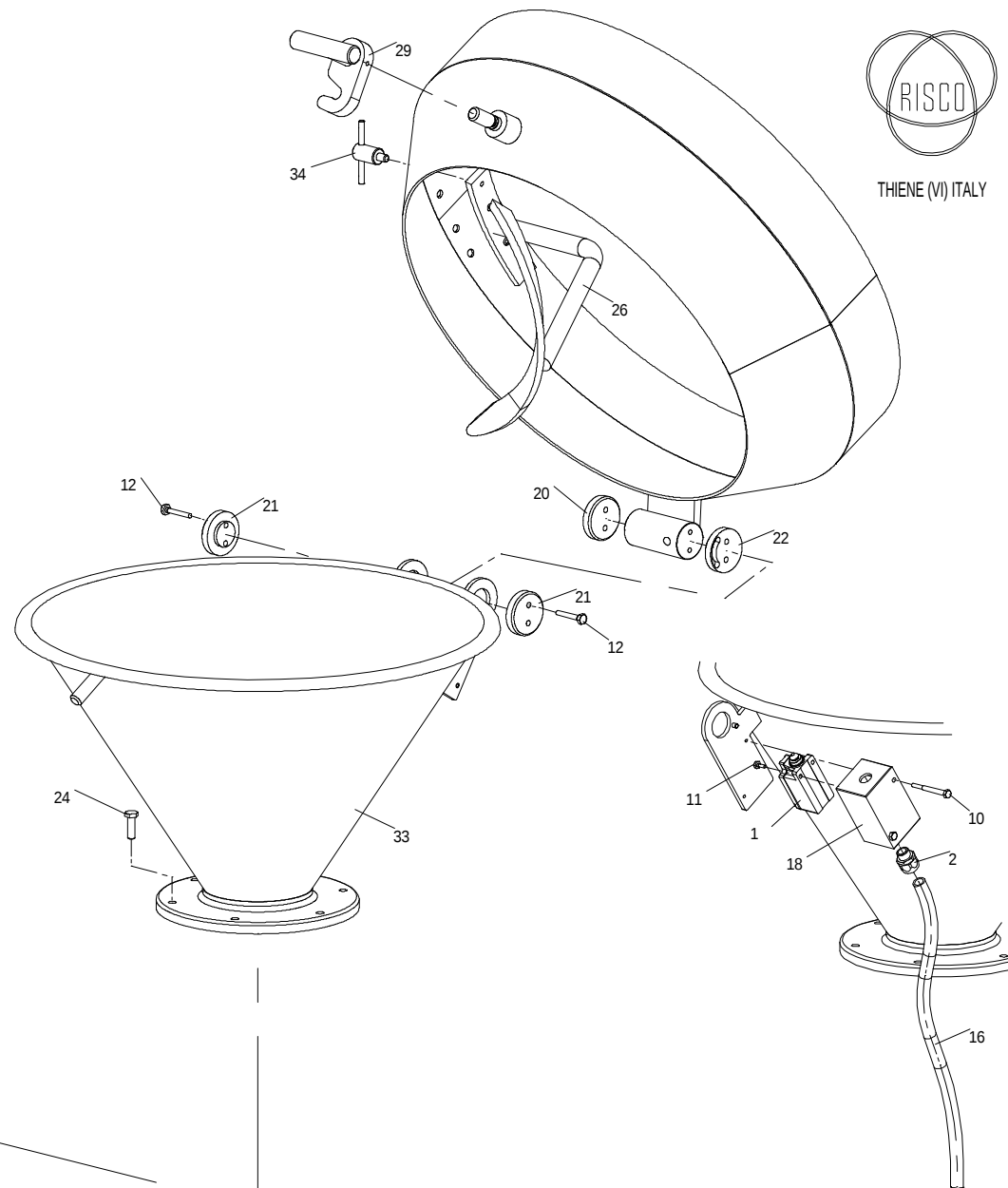
HOPPER GROUP
