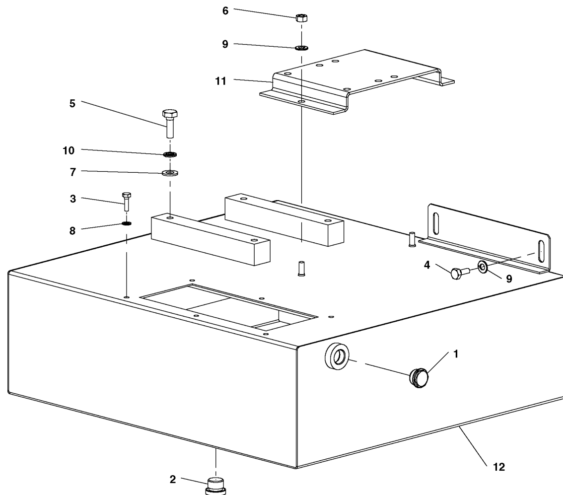
OIL TANK
