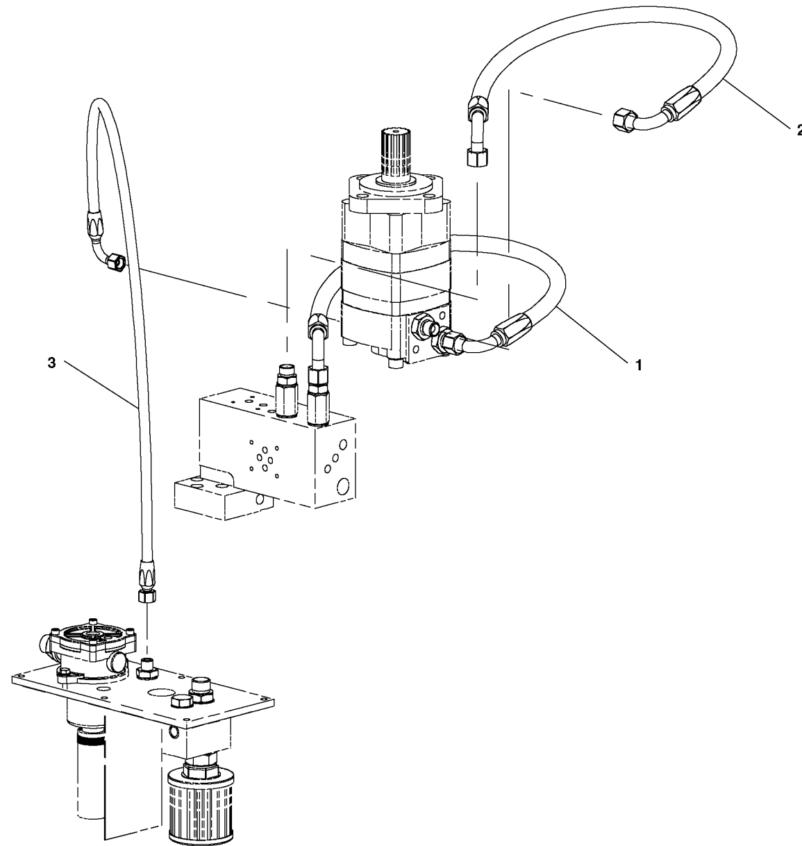
HYDRAULIC MOTOR HOSES CONNECTION
