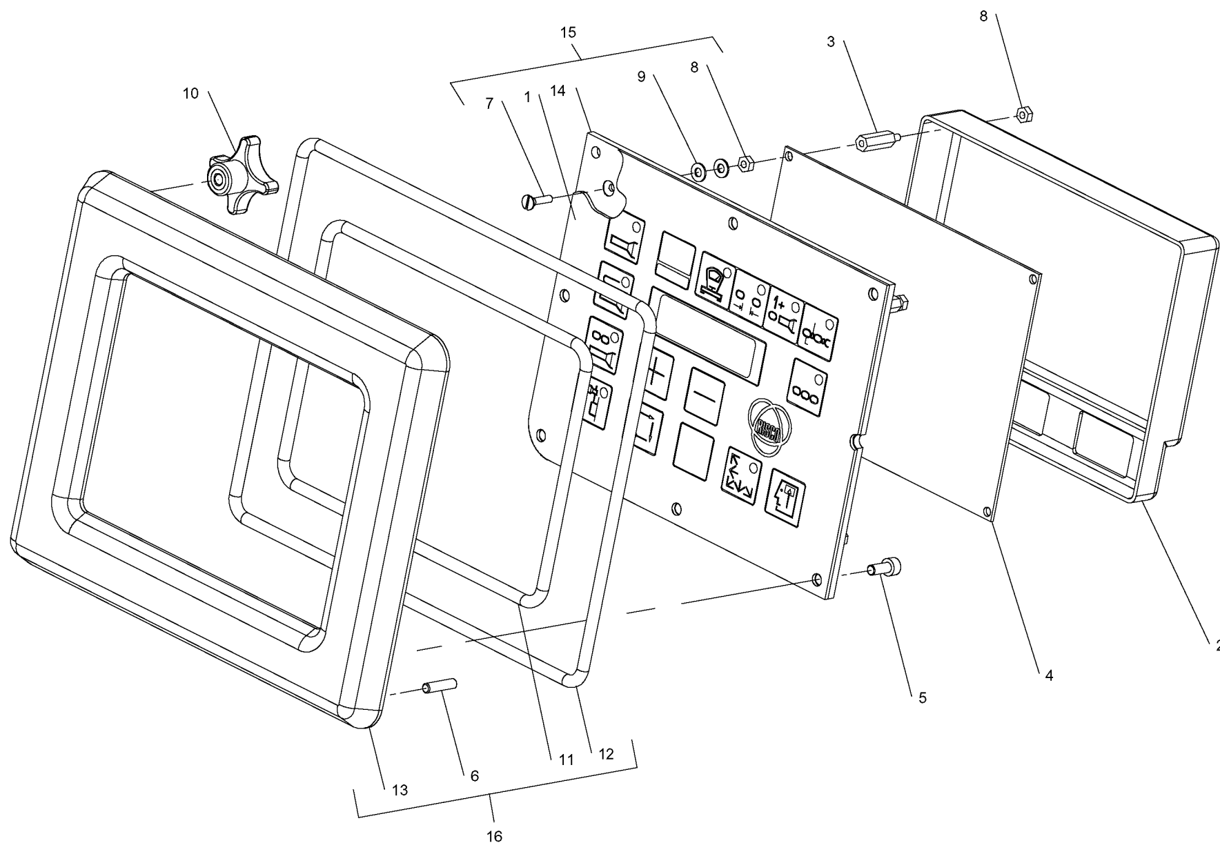
DIGITAL PANEL
