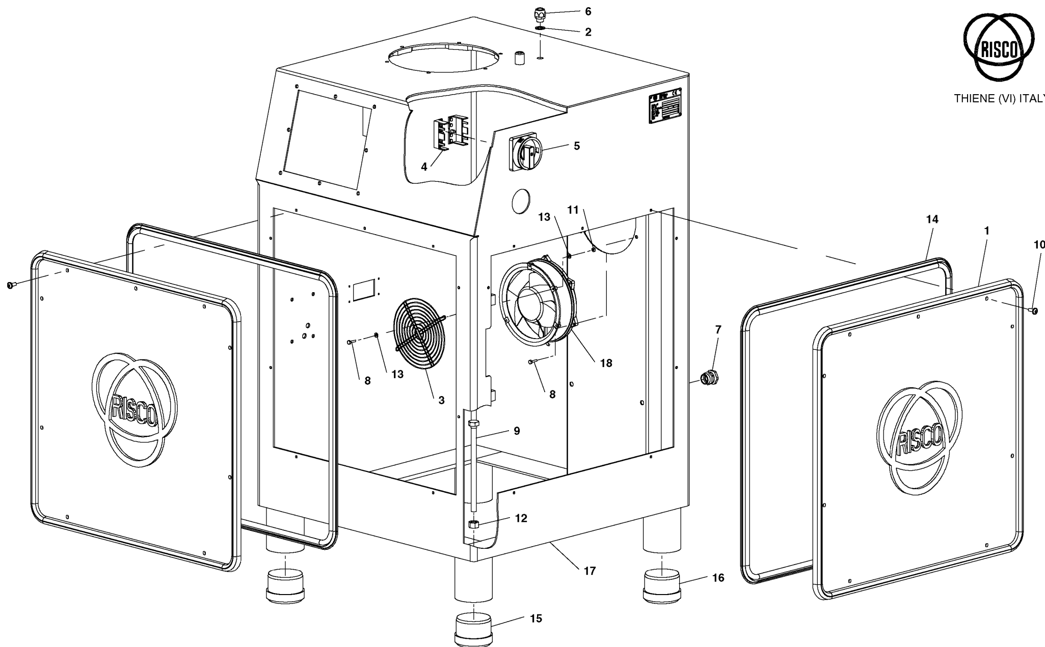
FRAME GROUP
