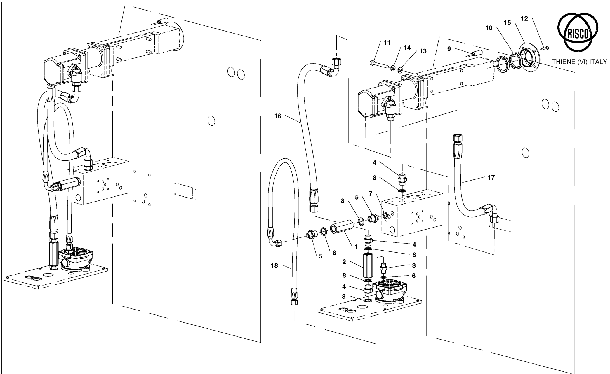
TWISTER CONNECTIONS
